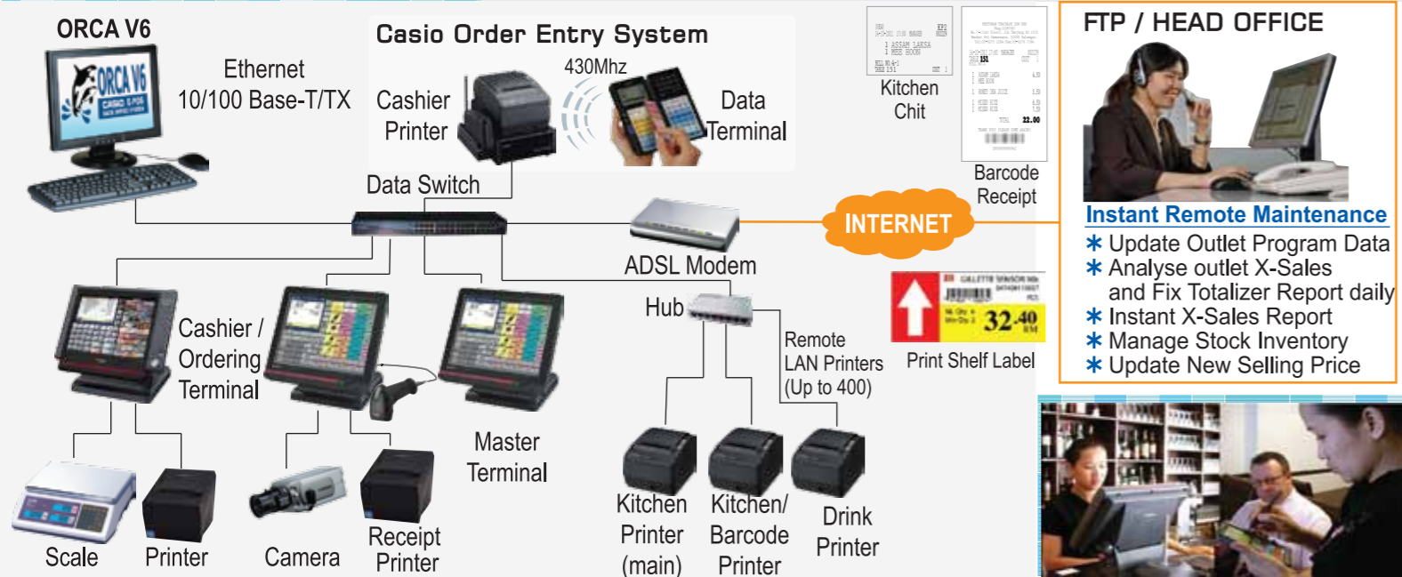
ORCA Stock Inventory System
